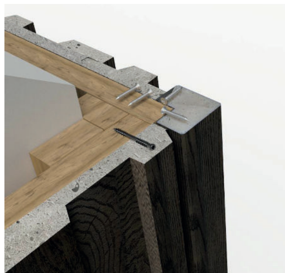
Fig. 8 - External corner detail
