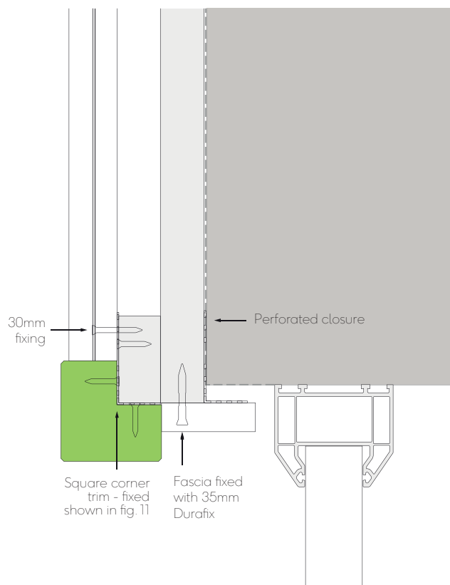
Fig. 13 - Window/door head with corner trim
