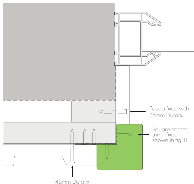
Fig. 12 - Window/door jamb with corner trim
