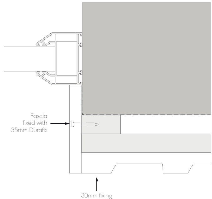
Fig. 14 - Window/door jamb with fascias
