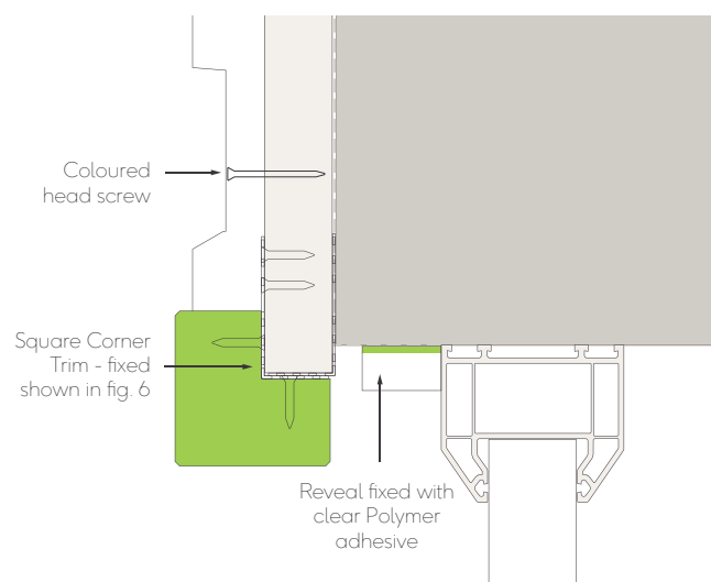
Fig. 12 - Window/door head with corner trim
