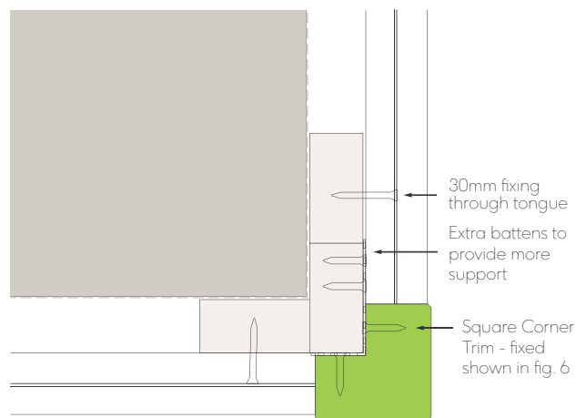
Fig. 8 - External corner detail
