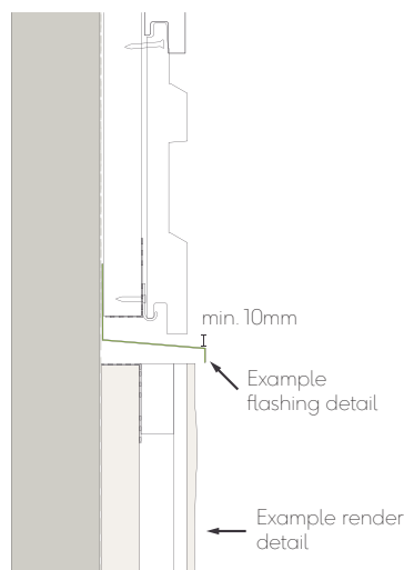
Fig. 22 - Installing cladding above render
