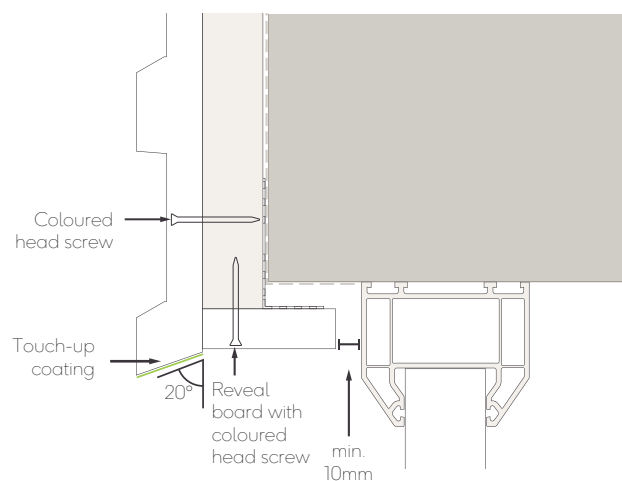
Fig. 13 - Window/door head with angled cut
