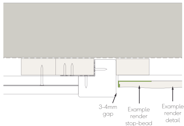
Fig. 20 - Corner profile butting up to render
