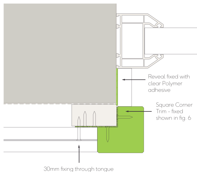
Fig. 11 - Window/door jamb with corner trim
